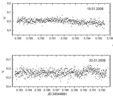
Fig. 1. Several daily light curves of SS Cyg obtained during the anomalous outburst in January 2008. Shown are the maximum of the outburst (the upper panel) and the declining part (the lower panel).
