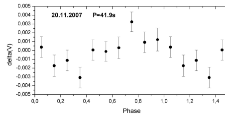
Fig. 4. Observations of SSCyg carried out in 2007 folded with the obtained period P=41.9 s. Observations are shown as filled circles, the vertical line denotes the mean \sigma
