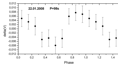
Fig. 5. Observations of SS Cyg folded with the P=98 s obtained in the 2008 data.
