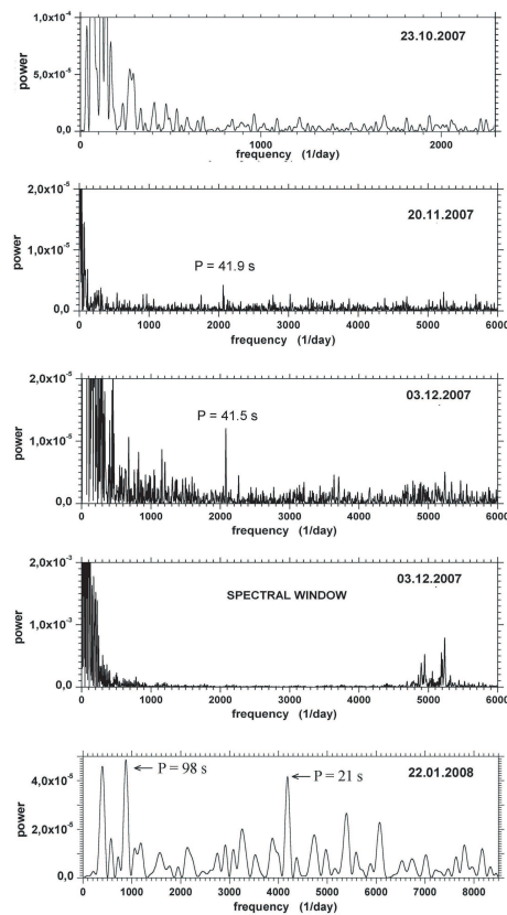
Fig. 3. Power spectra obtained for different nights from the analysis of SS Cyg observations in 2007–2008. The most prominent peaks are marked with arrows.
