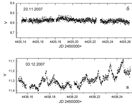
Fig. 2. The same is in Fig. 1 for the outburst observed in November 2007
